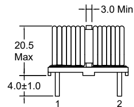
Orthographic view
