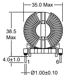
Orthographic view
