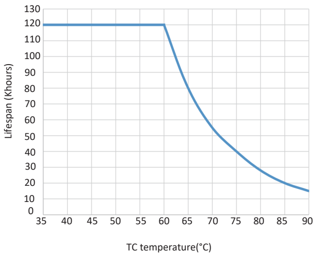
Lifespan vs TC temperature
